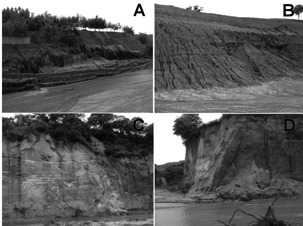
Fig. 2: Problems of erosion, collapse and mass movements associated with the presence of “Tierra Blanca Joven” (TBJ) tephras. (A) in spite of mitigation measures Las Cañas river affects regularly the slope; (B) recent rills in artificial landfill in Cumbres de San Bartolo, close to Las Cañas river; (C) lateral erosion, collapse, and slab failure in Las Cañas river; (D) lateral erosion, collapse, and slab failure in Las Cañas river, downstream of point of photo 3C.
