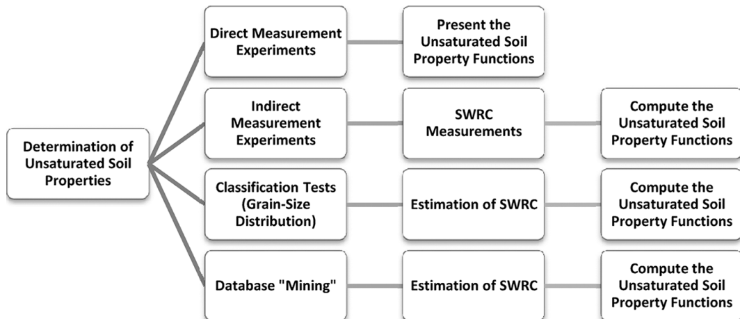
Fig. 4: Different approaches to obtain the unsaturated soil property functions (Fredlund et al., 2012).
