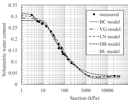
Fig. 13: Soil Water Retention Curve (SWRC) combining results of the filter paper and pressure plate, BC: Brooks & Corey ( \theta_s=0.28184 , \theta_r=0.018052 , a=12.522 , n=0.39281 , R^2=0.97796 ); VG: Van Genuchten ( \theta_s=0.29428 , \theta_r=0.032492 , \alpha=0.044737 , n=1.6255 , R^2=0.99093 ); LN: Kosugi ( \theta_s=0.30531 , \theta_r=0.037625 , \psi_m=55.468 , \sigma=1.5875 , R^2=0.99190 ); DB: Durner ( \theta_s=0.31389 , \theta_r=0.035789 , w_1=0.11533 , \alpha_1=0.27483 , n_1=6.7765 , \alpha_2=0.035362 , n_2=1.7162 , R^2=0.99517 ); BL: Seki ( \theta_s=0.31591 , \theta_r=0.039136 , w_1=0.084214 , \psi_m=3.1033 , \sigma_1=1.0456E-05 , \psi_m2=61.153 , \sigma_2=1.3983 , R^2=0.99388 ).
