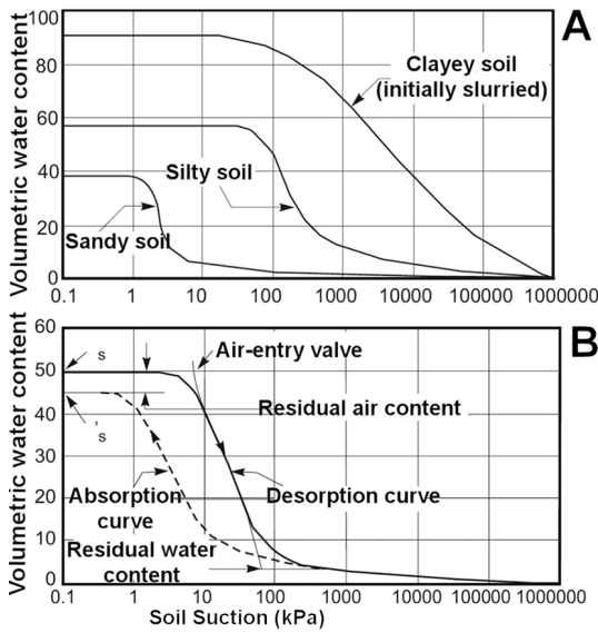
Fig. 3: (A) Typical Soil Water Retention Curves (SWRC) according to the soil type; (B) different stages and important concepts of the SWRC (Fredlund & Xing, 1994).
