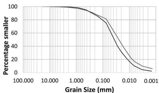
Fig. 1: Grain size curve range of the TBJ fall deposit, unit G (Pers. Comm. Of Ayala, O., 2013).
