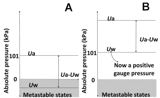
Fig. 8: Scheme of the axis translation technique that helps to avoid metastable states (Modified from Marinho et al., 2008). (A) Natural state: atmospheric conditions and negative water pore pressure; (B) After air pressure is injected into the system: axis-translation and positive water pore pressure.
