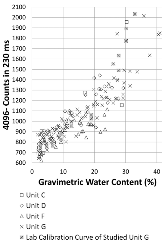
Fig. 16: Preliminary results of calibration curve using TMS1 in different units of TBJ of sectors of the Metropolitan Area of San Salvador (MASS).
