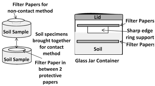
Fig. 7: Scheme used to assemble the filter paper tests (Modified from Bulut & Leong, 2008).
