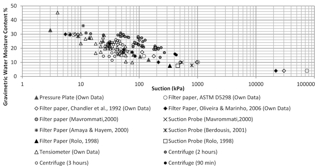
Fig. 6: TBJ Soil-Water Retention Curve (SWRC) of fall deposit of Unit "G" (Rolo et al., 2004) and own results using pressure plate, centrifuge, tensiometer and filter paper tests.
