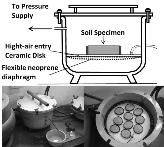
Fig. 9: Scheme (Agus et al., 2001) and photos of pressure plate test of TBJ samples.
