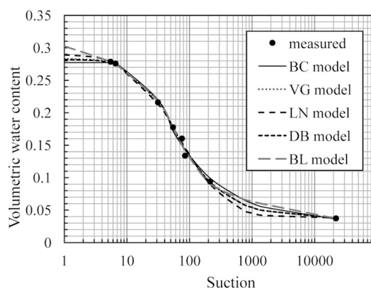
Fig. 12: Soil Water Retention Curve (SWRC) obtained with the filter paper, BC: Brooks & Corey ( \theta_s=0.27726 , \theta_r=0.029990 , a=18.986 , n=0.52604 , R^2=0.99461 ); VG: Van Genuchten ( \theta_s=0.28339 , \theta_r=0.035438 , \alpha=0.033343 , n=1.7346 , R^2=0.99651 ); LN: Kosugi ( \theta_s=0.28970 , \theta_r=0.038195 , \psi_m=65.629 , \sigma=1.4361 , R^2=0.99575 ); DB: Durner ( \theta_s=0.28243 , \theta_r=0.035742 , w_1=0.51201 , \alpha_1=0.033912 , n_1=1.6754 , \alpha_2=0.030620 , n_2=1.8391 , R^2=0.99646 ); BL: Seki ( \theta_s=0.42477 , \theta_r=0.0043722 , w_1=0.63683 , \psi_{m1}=2.3488 , \sigma_1=7.8678 , \psi_{m2}=57.498 , \sigma_2=0.88895 , R^2=0.99669 ).
