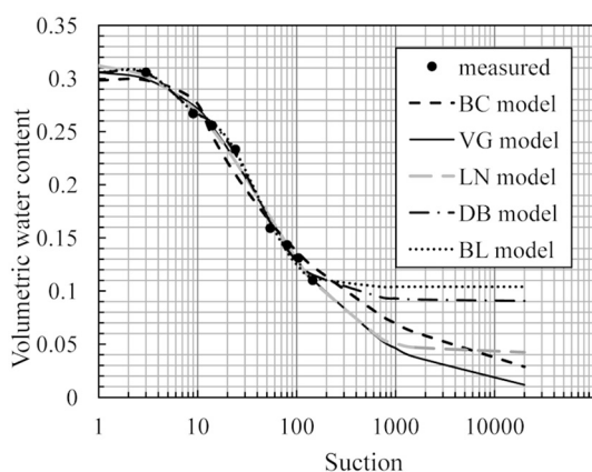
Fig. 11: Soil Water Retention Curve (SWRC) obtained with the pressure plate, BC: Brooks & Corey ( \theta_s=0.29829 , \theta_r=5.6867E-06 , a=7.3027 , n=0.29571 , R^2=0.97020 ); VG: Van Genuchten ( \theta_s=0.30737 , \theta_r=5.8751E-06 , \alpha=0.062125 , n=1.4588 , R^2=0.99090 ); LN: Kosugi ( \theta_s=0.31461 , \theta_r=0.042290 , \psi_m=47.166 , \sigma=1.6392 , R^2=0.99179 ); DB: Durner ( \theta_s=0.30583 , \theta_r=0.090617 , w_1=0.13135 , \alpha_1=0.24648 , n_1=48.250 , \alpha_2=0.036249 , n_2=2.2134 , R^2=0.99738 ); BL: Seki ( \theta_s=0.30596 , \theta_r=0.10396 , w_1=0.16406 , \psi_{m1}=4.8063 , \sigma_1=0.10872 , \psi_{m2}=41.138 , \sigma_2=0.77123 , R^2=0.99738 ).
