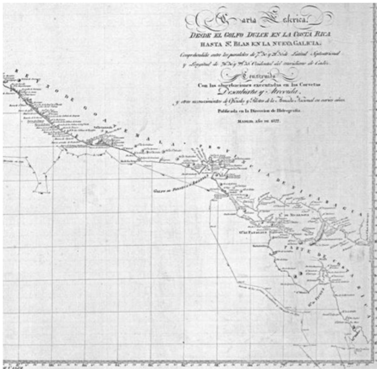
Figure 1. The Golfo Dulce to Caldera section of the Bauza chart (1822) Source: Martín-Meras, (1993), pp. 207-208.
